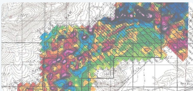
Figure 6: magnetic lows coincide with mapped veining and alteration.
